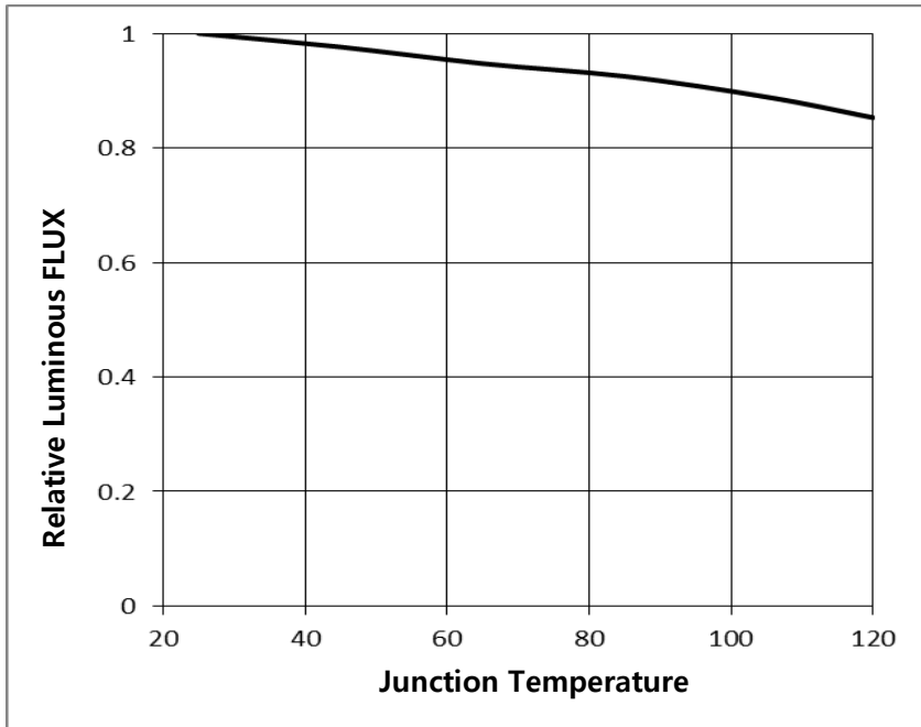
Fig 6. Junction Temperature vs. Relative Luminous FLUX, I_F=65mA
