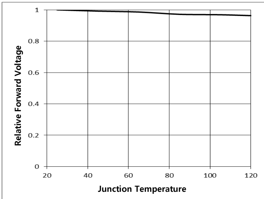
Fig 7. Junction Temperature vs. Relative Forward Voltage, I_F=65mA
