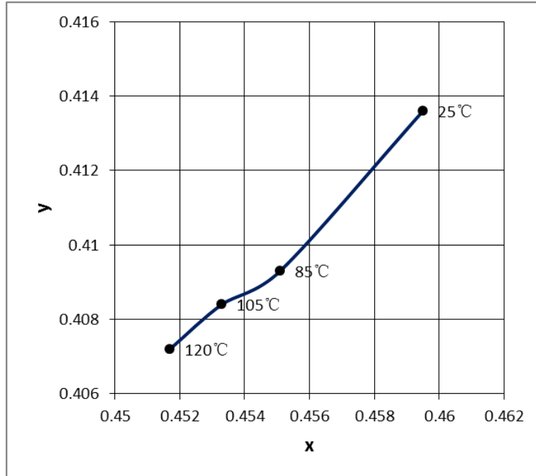
Fig 8. Chromaticity Coordinate vs. Junction Temperature, I_F=65mA (2600~4200K)
